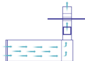
Classic Crossdraft booth air flow
